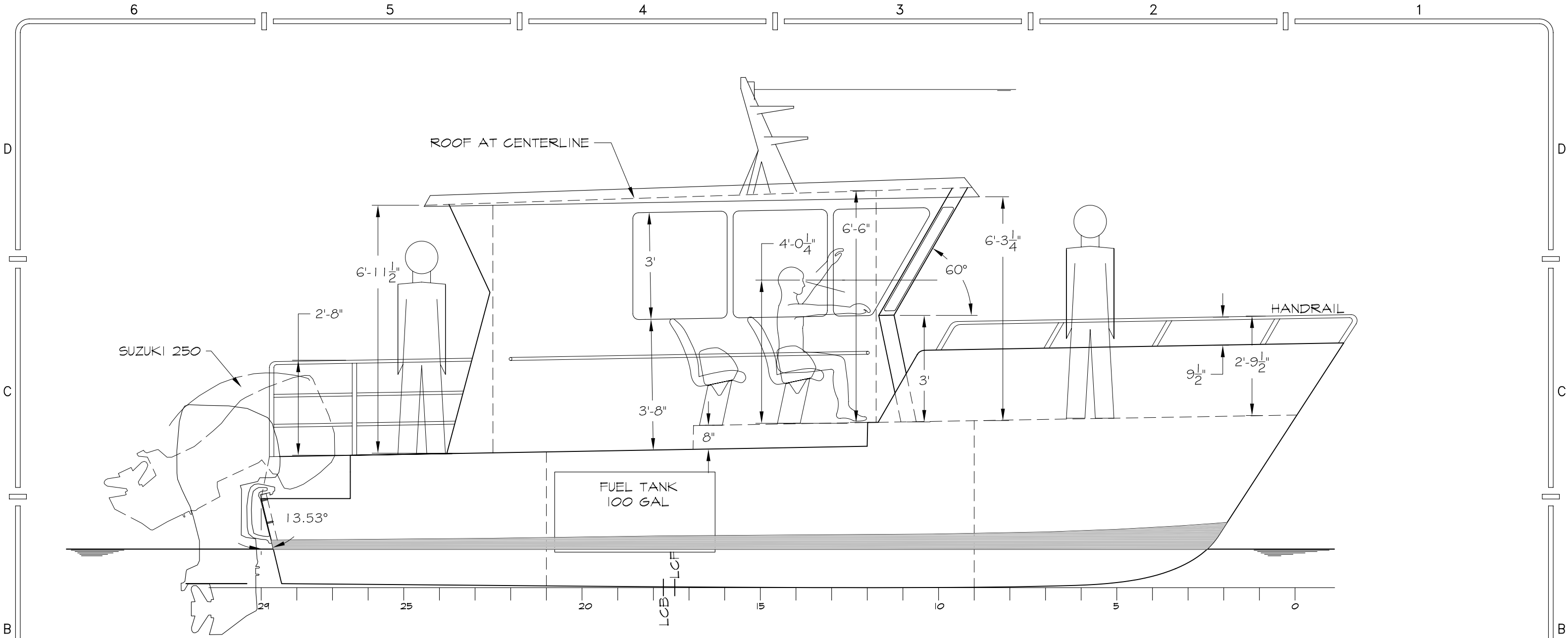
PROFILE Scale 3/8"=1'-0"
