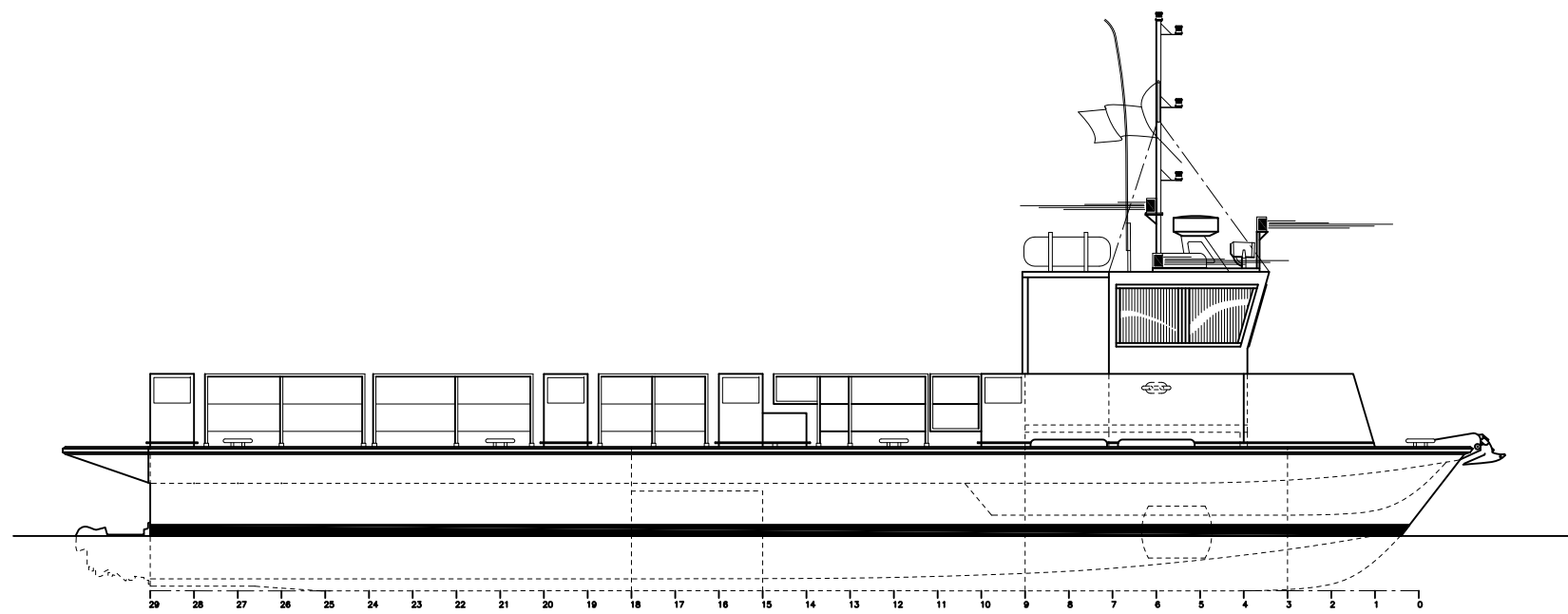
OUTBOARD PROFILE
