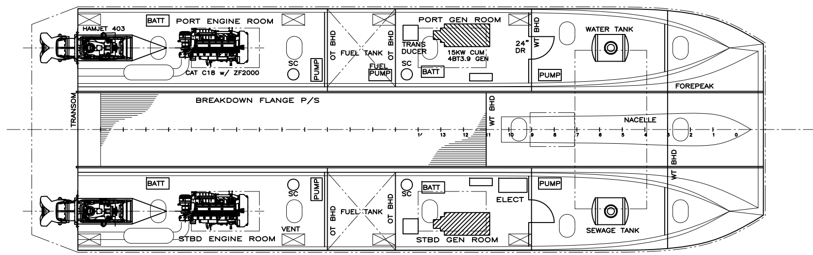
PLAN: BELOW DECK ARRANGEMENT
