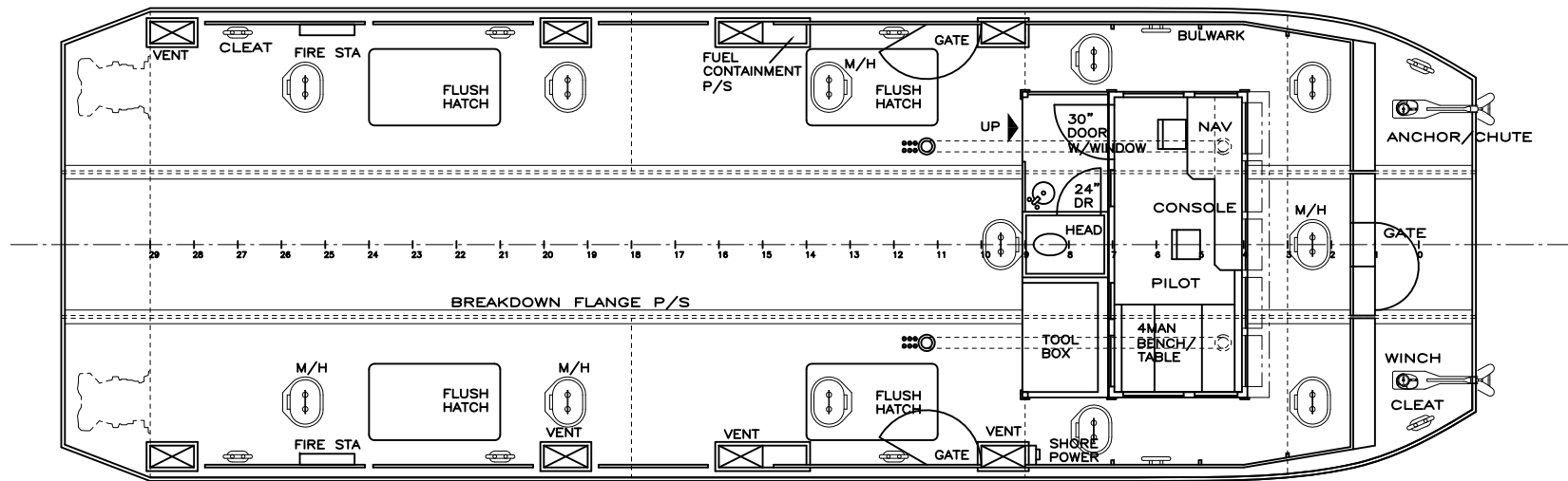
PLAN: MAIN DECK ARRANGEMENT
