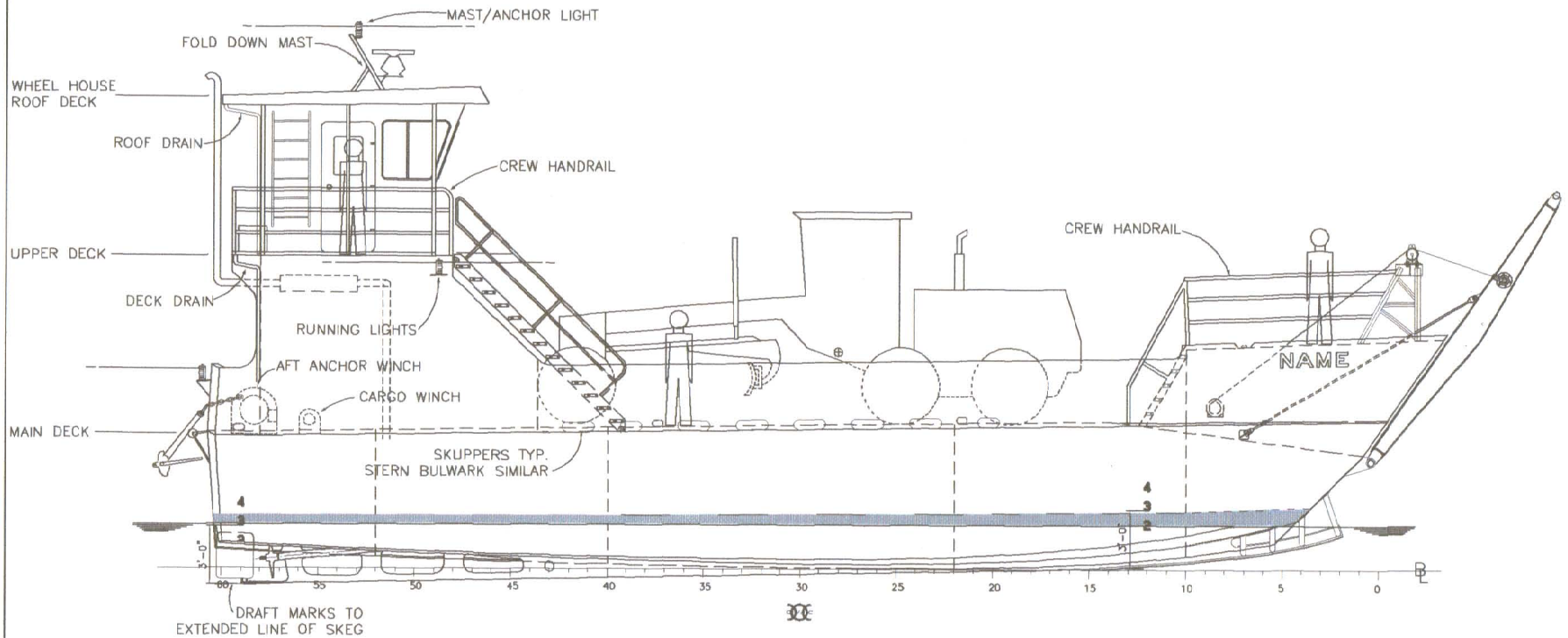
OUTBOARD PROFILE SCALE (A)
